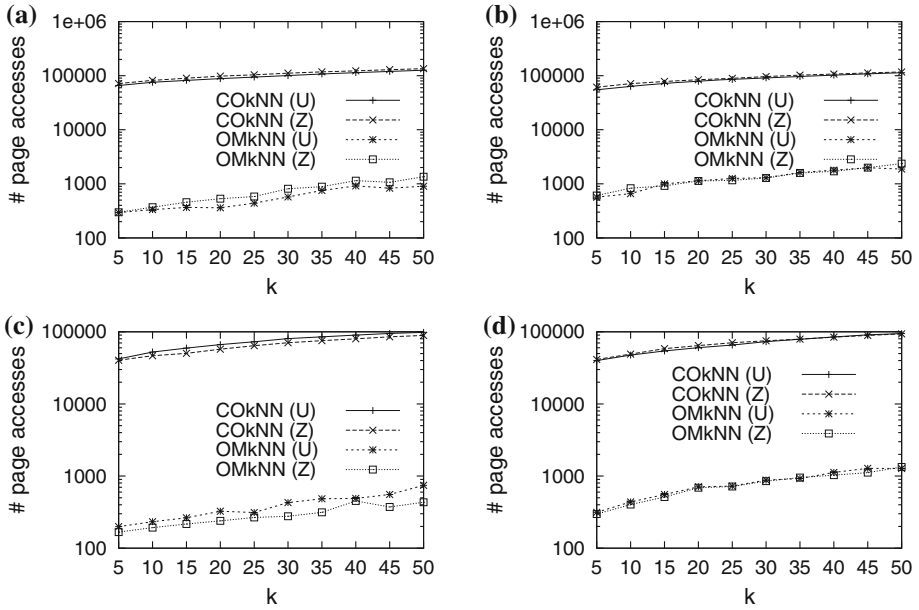
Fig. 15 Page accesses versus k
