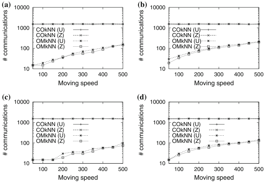
Fig. 23 Response time versus v_q
