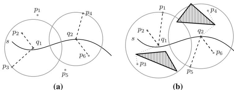
Fig. 1 Example of MkNN and obstructed MkNN
