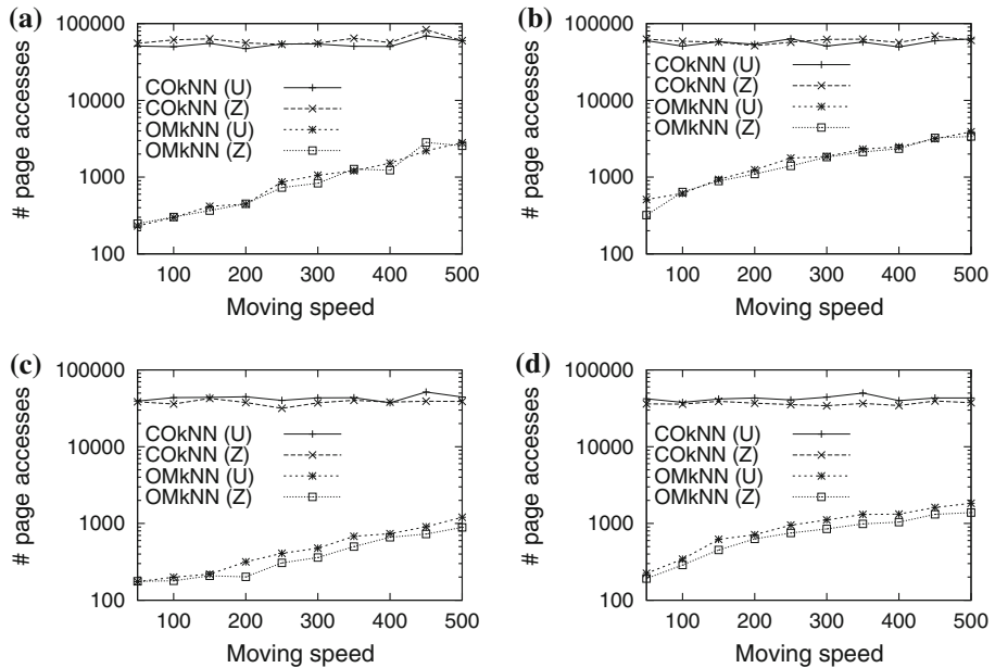
Fig. 22 Communications versus v_q
