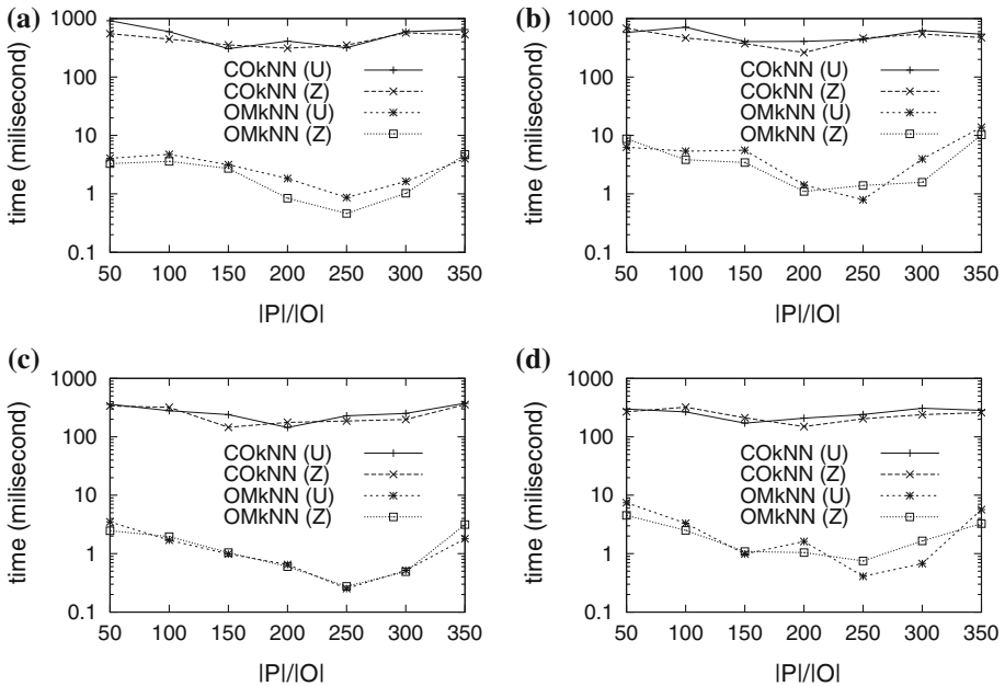
Fig. 20 Response time versus |P|/|O|
