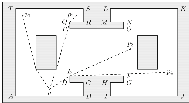
Fig. 13 Line segments as obstacles
