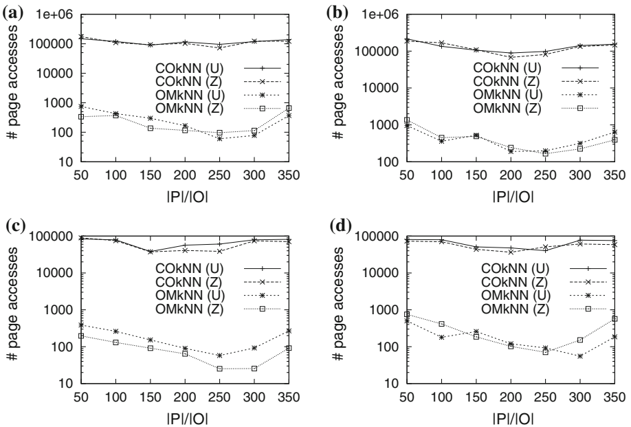
Fig. 18 Page accesses versus |P|/|O|
