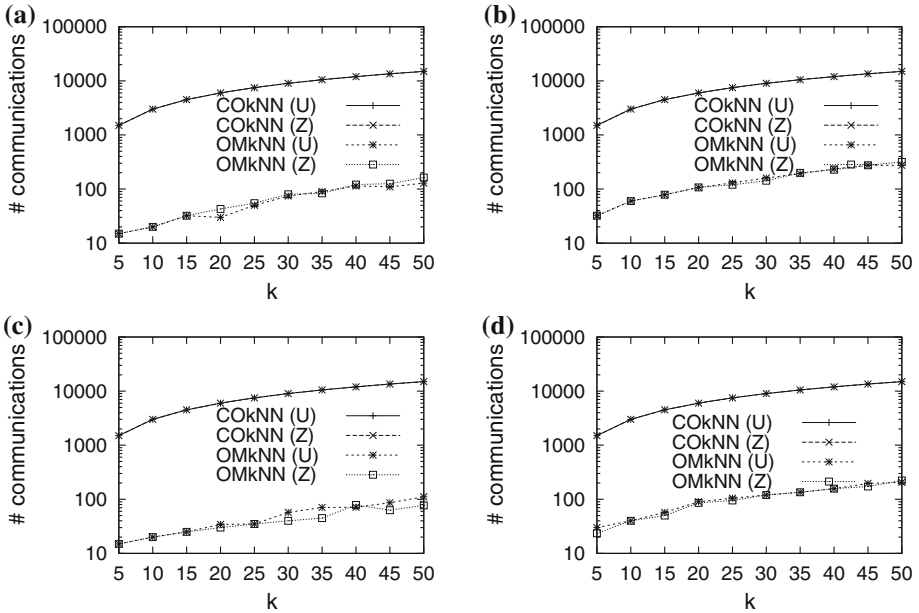
Fig. 16 Communications versus of k
