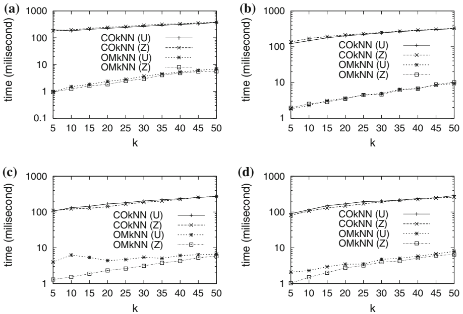
Fig. 17 Response time versus of k
