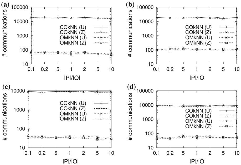
Fig. 19 Communications versus |P|/|O|
