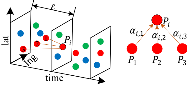
(b) Conv-intra operation. For each centroid point (e.g., P_i ), the neighborhoods of each point are defined as the points generated by the same sensor at earlier adjacent timestamps. In different local region, the number of neighborhoods is different, the order and the relative positions can be diverse. The feature of the centroid point is calculated as a weighted sum of neighborhoods' features. The points in different colors are generated by different sensors.
